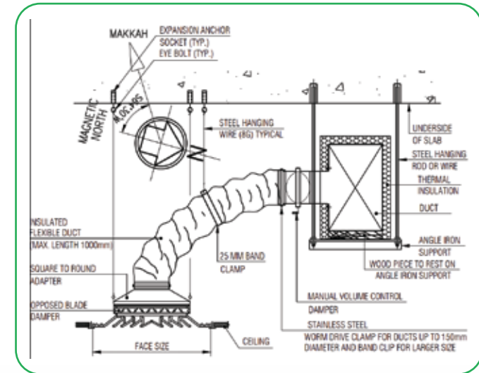
DIFFUSER INSTALLATION DETAIL
